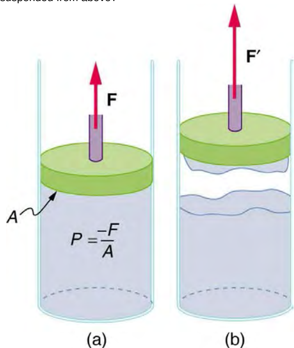
Figure 11.44 (a) When the piston is raised, it stretches the liquid slightly, putting it under tension and creating a negative absolute pressure P = -F/A . (b) The liquid eventually separates, giving an experimental limit to negative pressure in this liquid.
