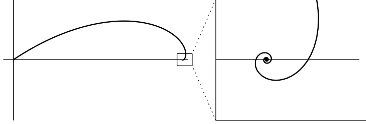
FIGURE 3. The curve defined by (5.12), for which the curvature approaches infinity at the free end. Although the curve has length one, its free end wraps around the limiting point \frac{3}{\sqrt{13}} infinitely many times. We have plotted this heuristically in the inset, although the actual curve wraps itself up too tightly for these loops to be visible.
