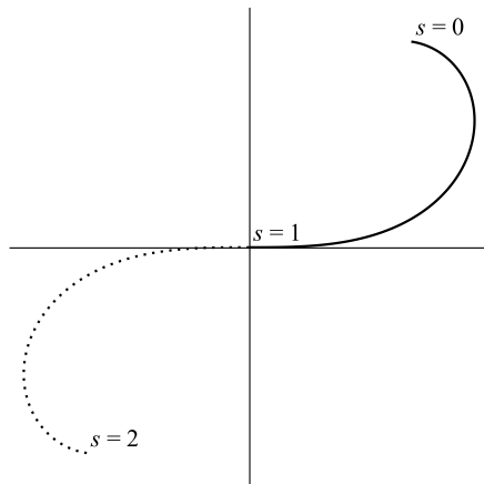
FIGURE 1. The free end of the curve is at s = 0 , while the fixed end is at s = 1 . We imagine the curve extending smoothly through the origin to s = 2 through an odd reflection such that \eta(s) = -\eta(1 - s) . Under such an extension, the tension extends to a smooth function satisfying \sigma(s) = \sigma(1 - s) .
