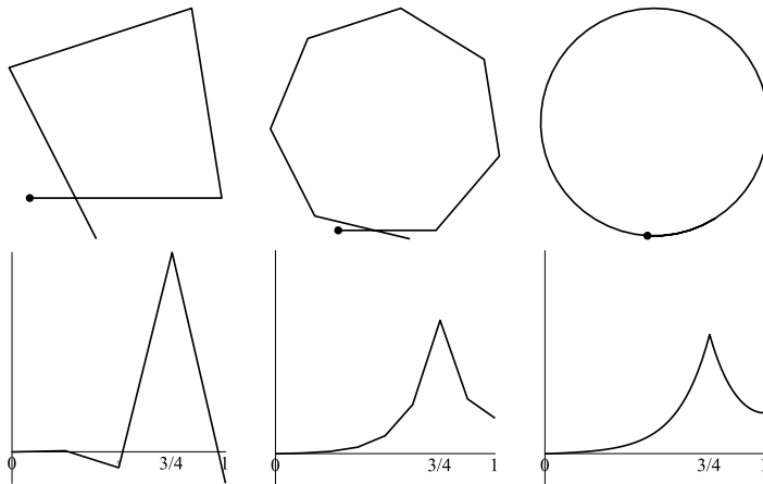
FIGURE 2. In the top row we plot chains with constant angles between consecutive segments, with n = 4 , n = 8 , and n = \infty links. In the bottom row we plot the corresponding discrete Green function G_{kj} as a function of \frac{k}{n} , evaluated at j = \frac{3n}{4} , for each configuration. Notice that when n = 4 the angles in the chain are acute, which is what allows the tension to become negative in that case. Also notice that as n \rightarrow \infty , the discrete Green function approaches the Green function for the differential equation.
