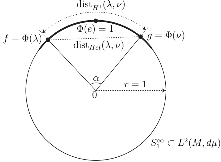
Figure 3.9. The Hellinger distance \text{dist}_{Hel}(\lambda, \nu) and the spherical Hellinger distance \text{dist}_{\dot{H}^1}(\lambda, \nu) between two points f = \Phi(\lambda) and g = \Phi(\nu) in S_1^\infty . The thick arc represents the image of \text{Diff}(M) under the map \Phi .
