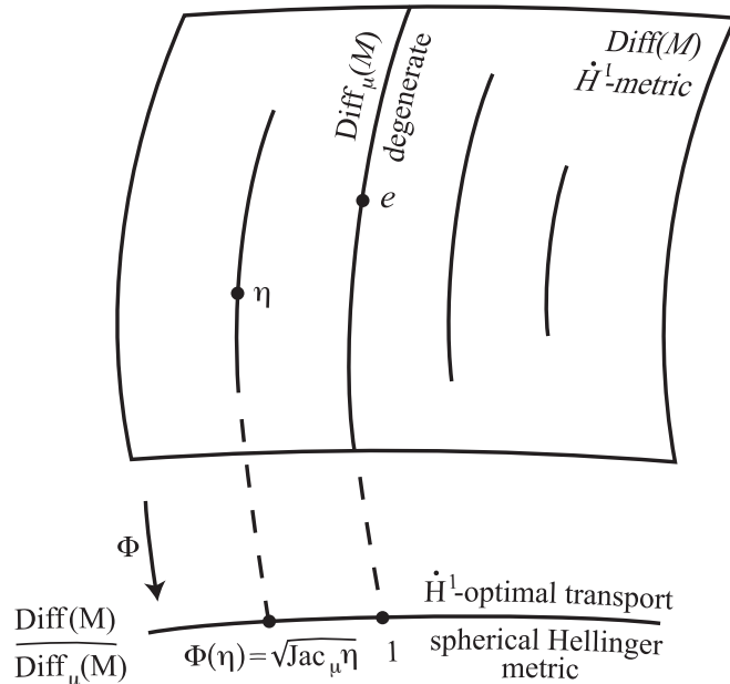
Figure 3.4. The fibration of \text{Diff}(M) with fiber \text{Diff}_\mu(M) determined by the reference density \mu together with the \dot{H}^1 -metric.
